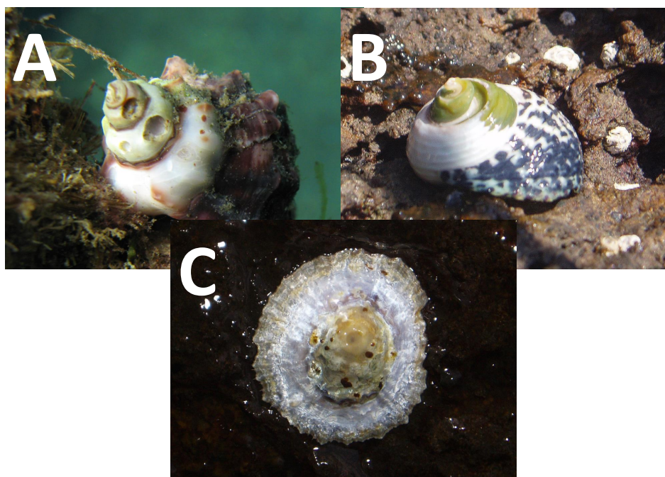
Fig. 1. Fig. 1 Gastropod molluscs living adjacent to shallow water CO 2 seeps off Ischia showing severely eroded shells due to the corrosive effects of the seawater a) Hexaplex trunculus , b) Osilinus turbinata
