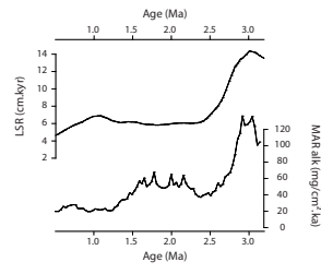
Figure 1. Smoother LSR and MAR alkenone concentration at the EEP Site 1239.
