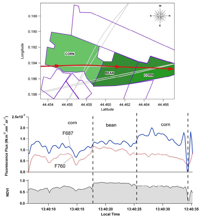
Fig. 10. Top: AirFLEX transects over the Marmande test fields on 15 September 2007. Bottom: Fluorescence flux at 687 nm, fluorescence flux at 760 nm and NDVI measured during the transect marked in red.
