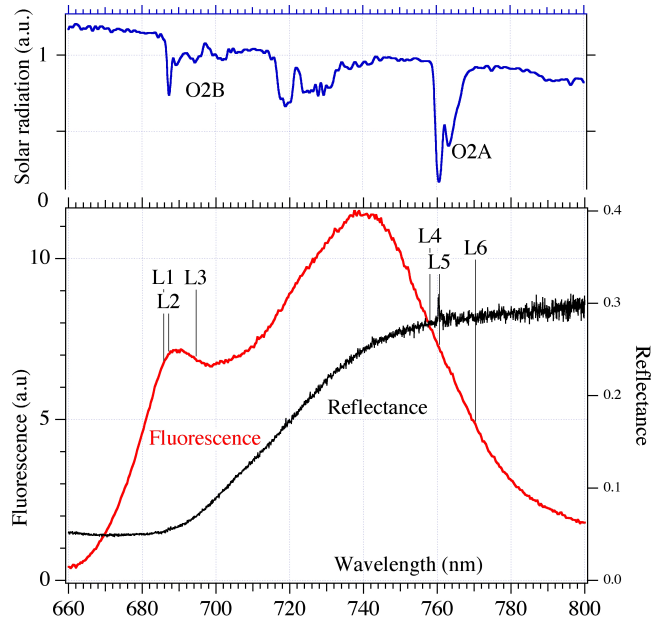
Fig. 2. Top: Solar spectrum showing the O 2 bands at the spectral resolution of the AirFLEX sensor. Bottom: Red and near-infrared region of the fluorescence emission spectrum after full sun light adaptation of a Velvetgrass leaf. Sun-induced fluorescence was measured with the special instrument described in Sect. 2.1.3. The reflectance spectrum has been superimposed. It was acquired at the canopy level with the SpectroFLEX set-up. The positions of the central wavelengths (Li) of the six channels of the AirFLEX sensor are also shown. These spectra were required to retrieve the fluorescence by the FLD principle.
