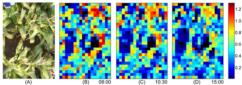
Fig. 8. (A) Corn canopy area (about 1\text{ m}^2 ) scanned by the FLIDAR imaging system, within small angles from nadir; note the presence of a fluorescence standard (blue) and a reflectance standard (white) at the left-top corner. (B–D) Canopy fluorescence maps at the 760 nm band, with excitation at 532 nm, acquired in sequence at 08:00, 10:30 and 15:00 UTC, respectively, on 12 September 2007. Each map, made up of 18 \times 27 pixels, required an acquisition time of 20 min. Fluorescence intensities in the colour bar are expressed as arbitrary units.
