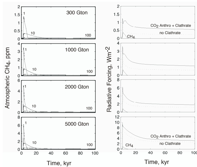
Fig. 2. Model projection of the radiative impact of a fossil fuel CO 2 release over the coming 100 kyr, from Archer and Buffett (2005). (a) The warming from the CO 2 (300, 1000, 2000, and 5000 Gton releases) provokes methane to degas from the ocean hydrate reservoir, increasing the methane concentration during the time interval that the methane is released. The methane is oxidized and accumulates in the atmosphere. (b) Radiative impacts of the CO 2 and methane releases. The methane direct effect is smaller than the original CO 2 radiative forcing, and it is also smaller and much shorter-lived than the radiative effect of the oxidized methane as CO 2 , gauged the difference between the anthropogenic CO 2 radiative forcing with and without clathrate feedback. The point of the figure is to show that the greatest impact from a slow, ongoing methane release may be from the accumulation of its oxidation product, CO 2 .
