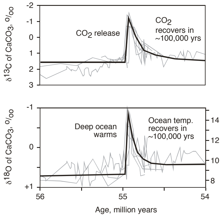
Fig. 7. Carbon and oxygen isotopic excursion known as the Paleocene Eocene Thermal Maximum, from Zachos et al. (2001).
