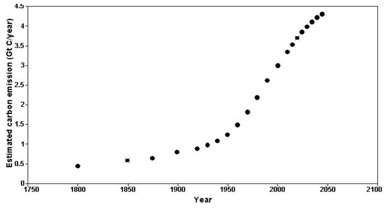
Fig. 1. Estimated direct and indirect metabolic CO 2 release from pre-industrial to year 2050.
