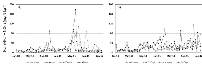
Figure 2. Mineral nitrogen contents [ \text{mg N kg}^{-1} ] for the arable land (a) and the grassland (b) of the soil depth 0–10 cm for the years 2010 and 2011.
