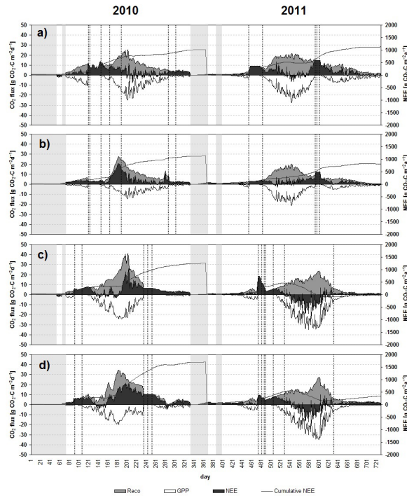
Figure 5. Time series of modeled \text{CO}_2 fluxes [ \text{gCO}_2\text{-Cm}^{-2}\text{d}^{-1} ] and cumulative NEE [ \text{gCO}_2\text{-Cm}^{-2}\text{yr}^{-1} ] for each site in 2010 and 2011; (a) arable land, 2010 maize, 2011 oat, C_{\text{medium}} ; (b) arable land, 2010 maize, 2011 oat, C_{\text{high}} ; (c) arable land, 2010 oat, 2011 maize, C_{\text{medium}} ; (d) arable land, 2010 oat, 2011 maize, C_{\text{high}} . Grey bars mark the period with snow cover. Dashed lines indicate management activities (see Table 2).
