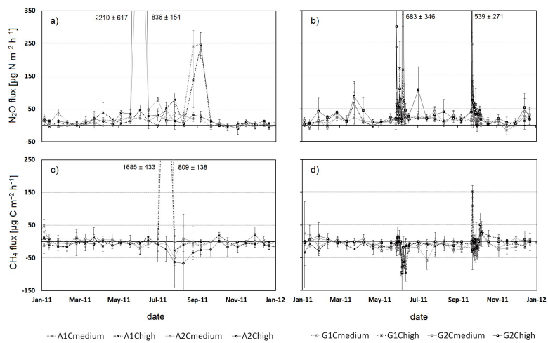
Figure 7. Time series of measured N_2O fluxes (a, arable land; b, grassland) and CH_4 fluxes (c, arable land; d, grassland) for the year 2011.
