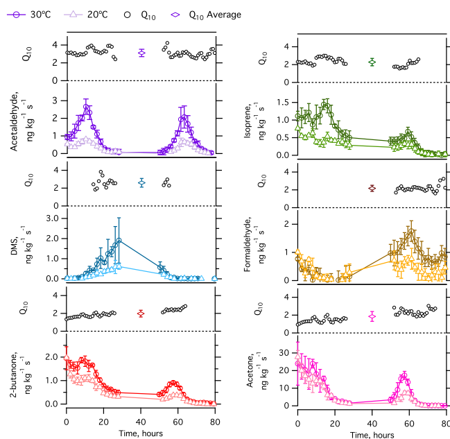
Figure 3. VOC emission observed from the Suriname rainforest (SR) soil sample. Soil temperature was modulated between 20 °C (colored triangles) and 30 °C (colored circles) to determine the temperature amplification factor, Q_{10} value (black markers), which can be used to separate microbial and abiotic processes driving the emission of VOC. The colored diamonds represent the average Q_{10} value for entire experiment \pm one standard deviation.
